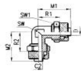
MODEL B219 TUBE (METRIC) - THREAD
