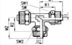
MODEL B218 (RPUT) TUBE (METRIC) - THREAD
