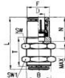
MODEL B112 (MPM)
