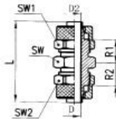
MODEL B216 (RPUC) TUBE (METRIC) - THREAD
