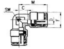
MODEL B113 (MPUL)
